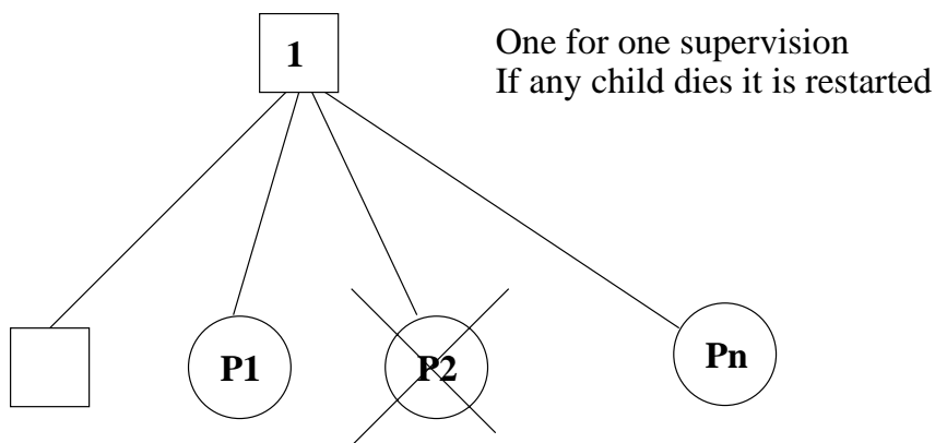
Figure 1.3: One_For_One Supervision
