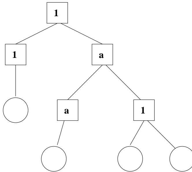
Figure 1.1: Supervision Tree
